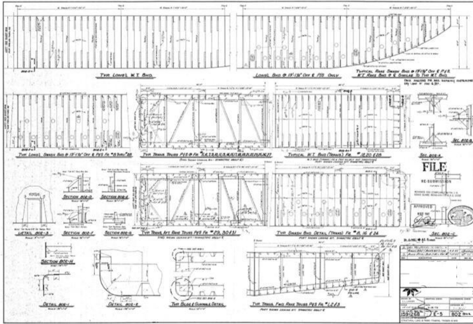
ABS Drawing (Framing Layout)
